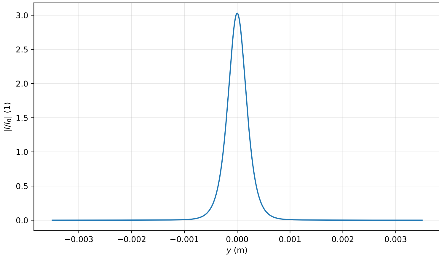
Intensity profile I(x=0, y, z=3.582)/I_0 , P_{in}=1.0P_{cr} , artificial time
